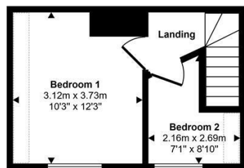
First Floor Approx 20 sq m / 216 sq ft
